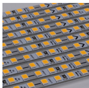
12V 27.7mm cut 9W/m Ra80+ 152LED/m
