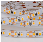
12V 12.5mm cut 10W/m Ra90+ 240LED/m Dotless
