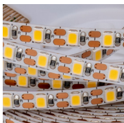
12V 8.33mm cut 10W/m Ra90+ 60LED/m
