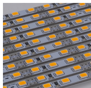
12V 25mm cut 16W/m Ra90+ 120LED/m Dotless
