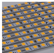
12V 27.7mm cut 9W/m Ra80+ 152LED/m
