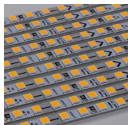
12V 27.7mm cut 9W/m Ra80+ 152LED/m Dotless
