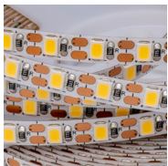
12V 8.33mm cut 10W/m CRI 90 120LED/m Dotless
