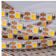
12V 8.33mm cut 10W/m Ra90+ 120LED/m
