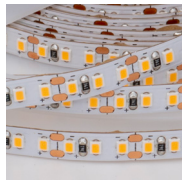
12V 12.5mm cut 10W/m CRI 90 240LED/m Dotless
