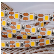
24V 8.33mm cut 16W/m Ra90+ 120LED/m
