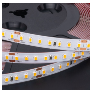
24V 50mm cut 18W/m*2line Ra90+ 280LED/m Dotless
